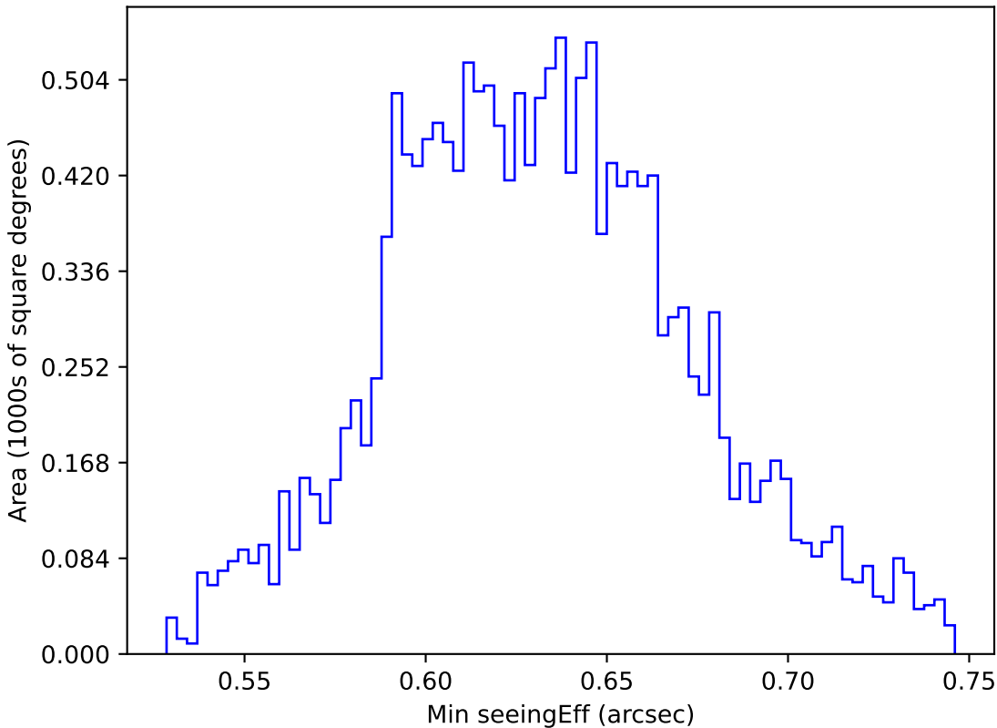
ddf_acor_sf30_lsf40_lsr20_v3.4_10yrs WFD y band: Min seeingEff
