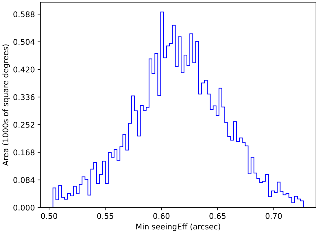
ddf_acor_sf30_lsf40_lsr20_v3.4_10yrs WFD r band: Min seeingEff
