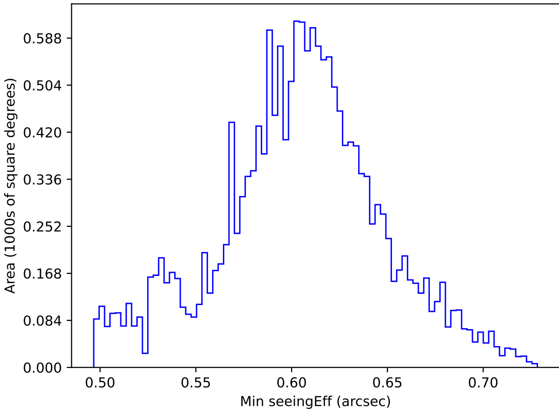
ddf_acor_sf30_lsf40_lsr20_v3.4_10yrs WFD i band: Min seeingEff
