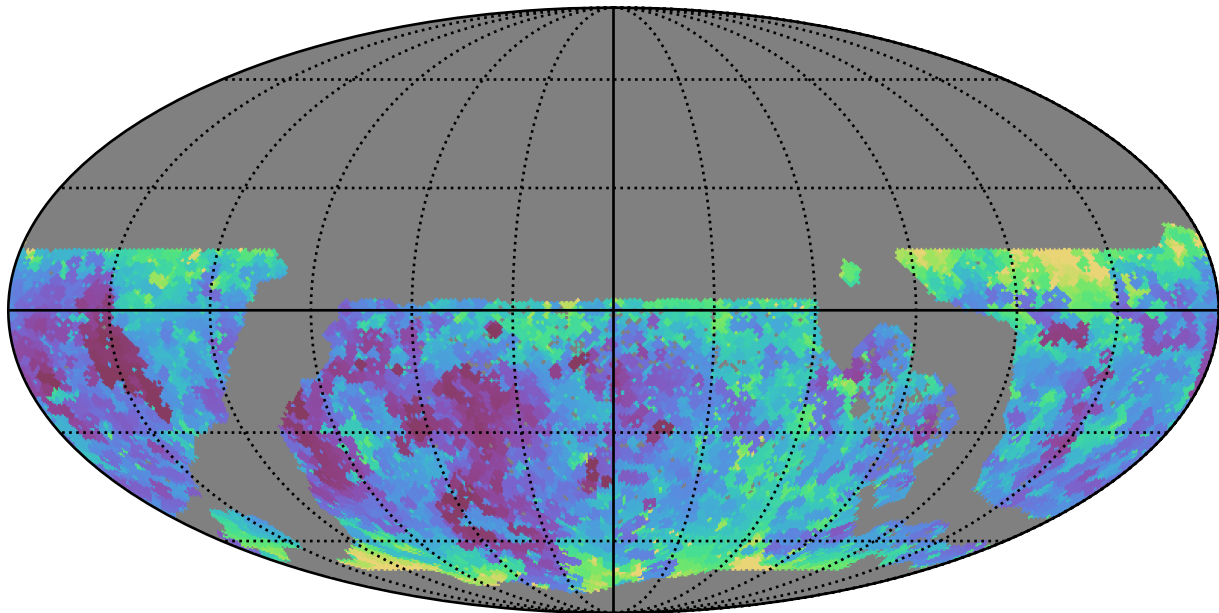
ddf_acor_sf30_lsf40_lsr20_v3.4_10yrs WFD g band: Min seeingEff
