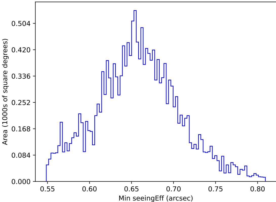
ddf_acor_sf30_lsf40_lsr20_v3.4_10yrs WFD g band: Min seeingEff
