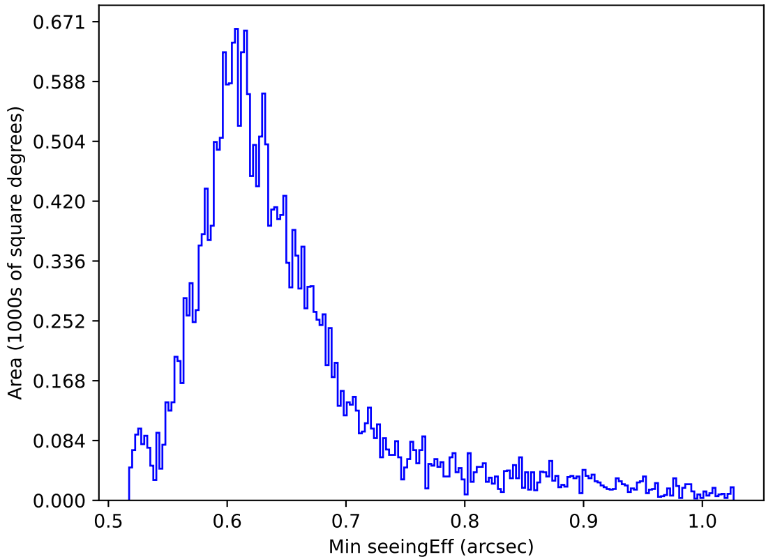
ddf_acor_sf30_lsf40_lsr20_v3.4_10yrs All sky z band: Min seeingEff
