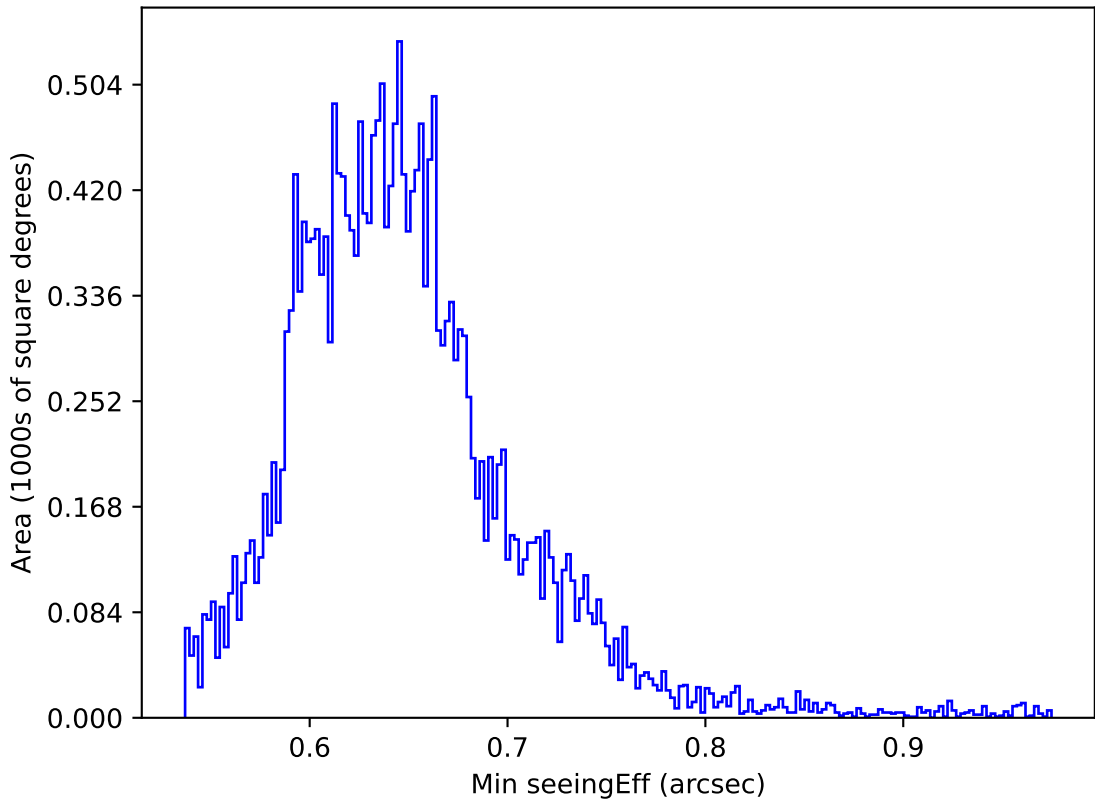
ddf_acor_sf30_lsf40_lsr20_v3.4_10yrs All sky y band: Min seeingEff
