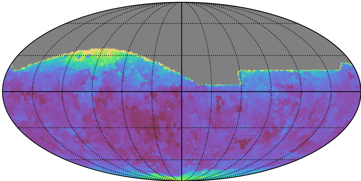
ddf_acor_sf30_lsf40_lsr20_v3.4_10yrs All sky r band: Min seeingEff
