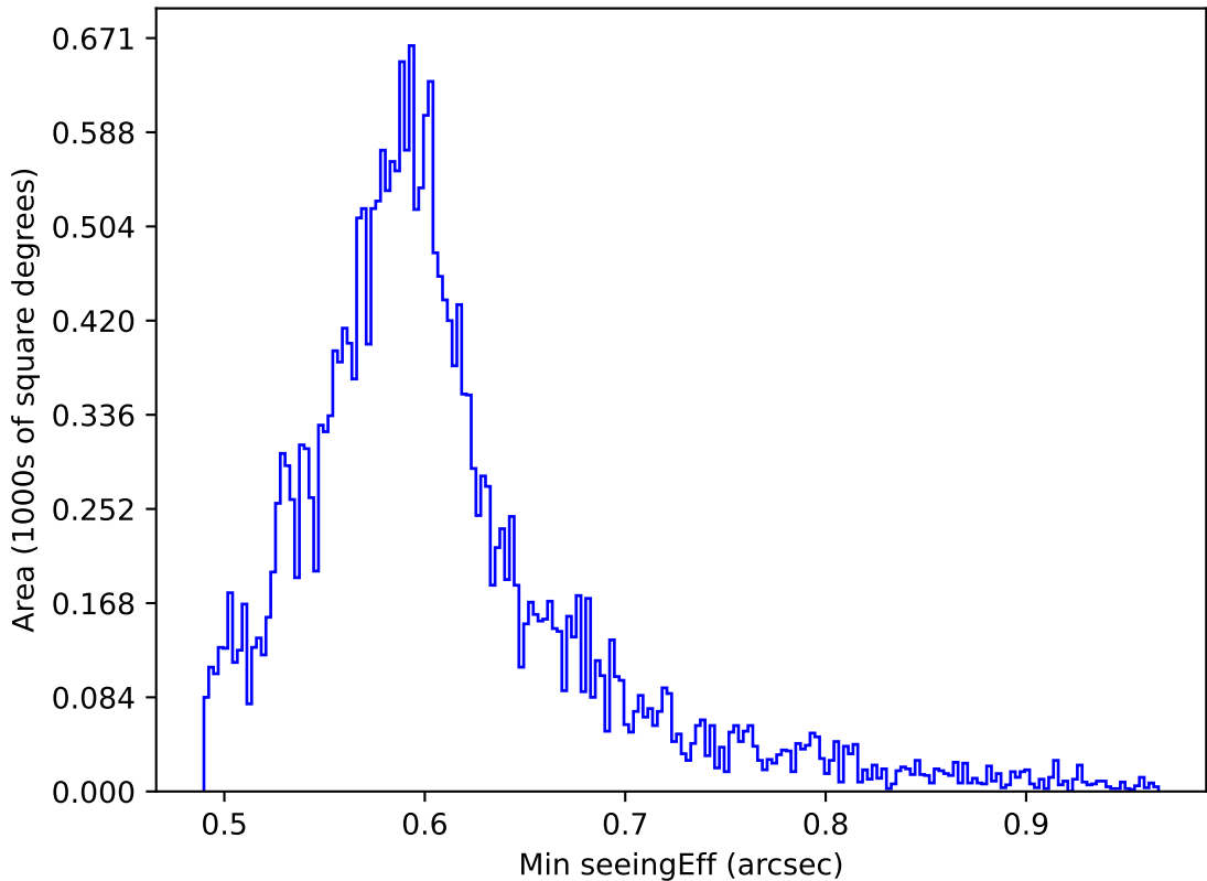
ddf_acor_sf30_lsf40_lsr20_v3.4_10yrs All sky all bands: Min seeingEff
