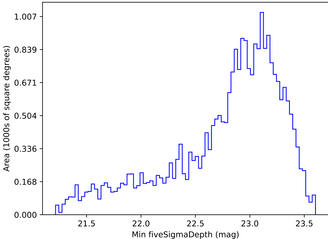
ddf_acor_sf30_lsf40_lsr20_v3.4_10yrs Yr 1 i band: Min fiveSigmaDepth
