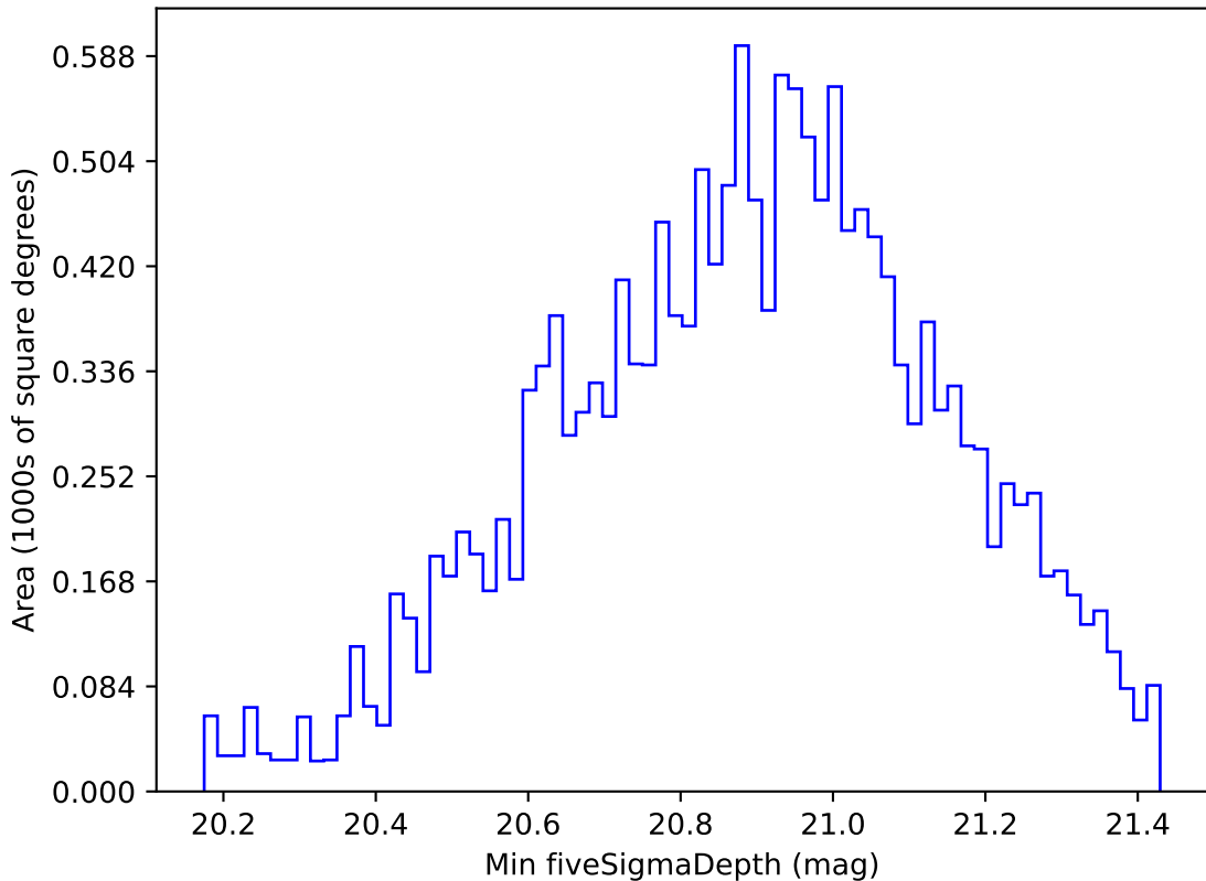
ddf_acor_sf30_lsf40_lsr20_v3.4_10yrs WFD y band: Min fiveSigmaDepth
