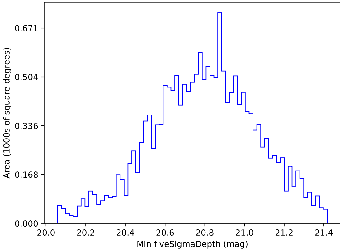
ddf_acor_sf30_lsf40_lsr20_v3.4_10yrs WFD all bands: Min fiveSigmaDepth
