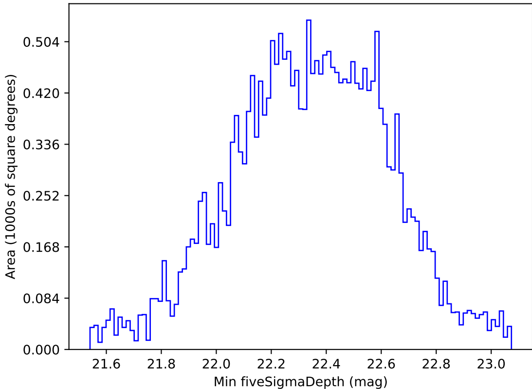
ddf_acor_sf30_lsf40_lsr20_v3.4_10yrs All sky u band: Min fiveSigmaDepth
