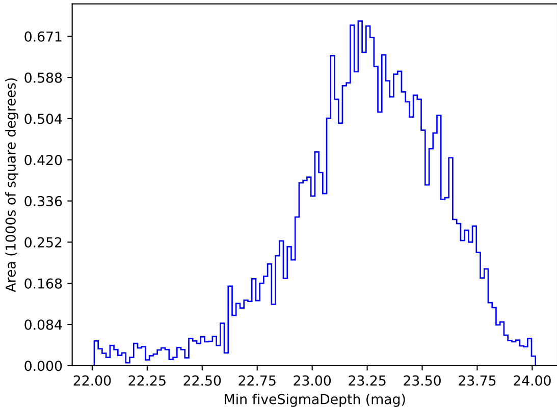
ddf_acor_sf30_lsf40_lsr20_v3.4_10yrs All sky g band: Min fiveSigmaDepth
