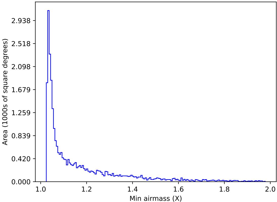
ddf_acor_sf30_lsf40_lsr20_v3.4_10yrs Yr 1 r band: Min airmass
