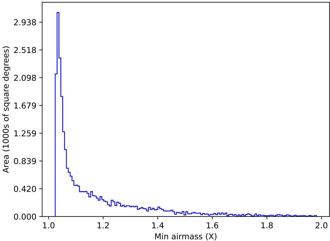
ddf_acor_sf30_lsf40_lsr20_v3.4_10yrs Yr 1 i band: Min airmass
