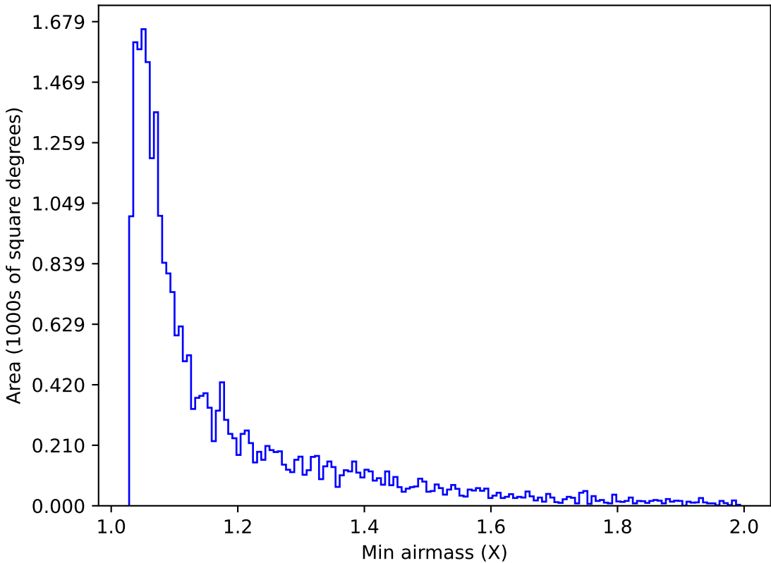
ddf_acor_sf30_lsf40_lsr20_v3.4_10yrs Yr 1 g band: Min airmass
