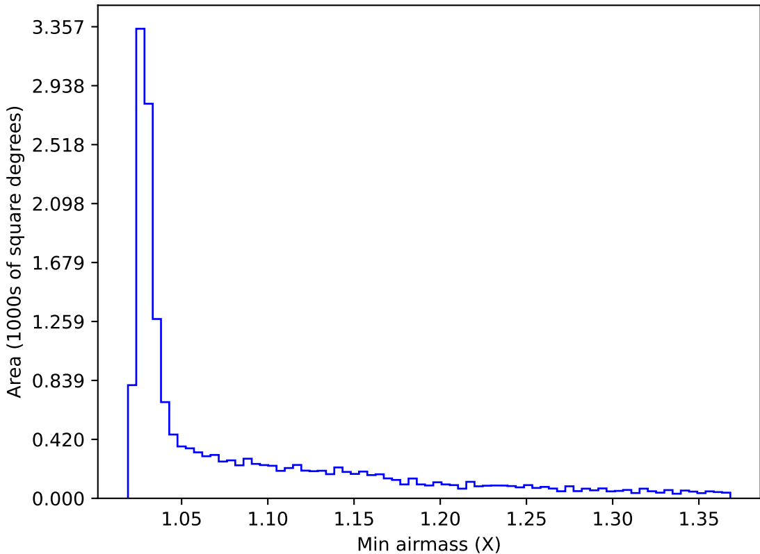
ddf_acor_sf30_lsf40_lsr20_v3.4_10yrs WFD z band: Min airmass
