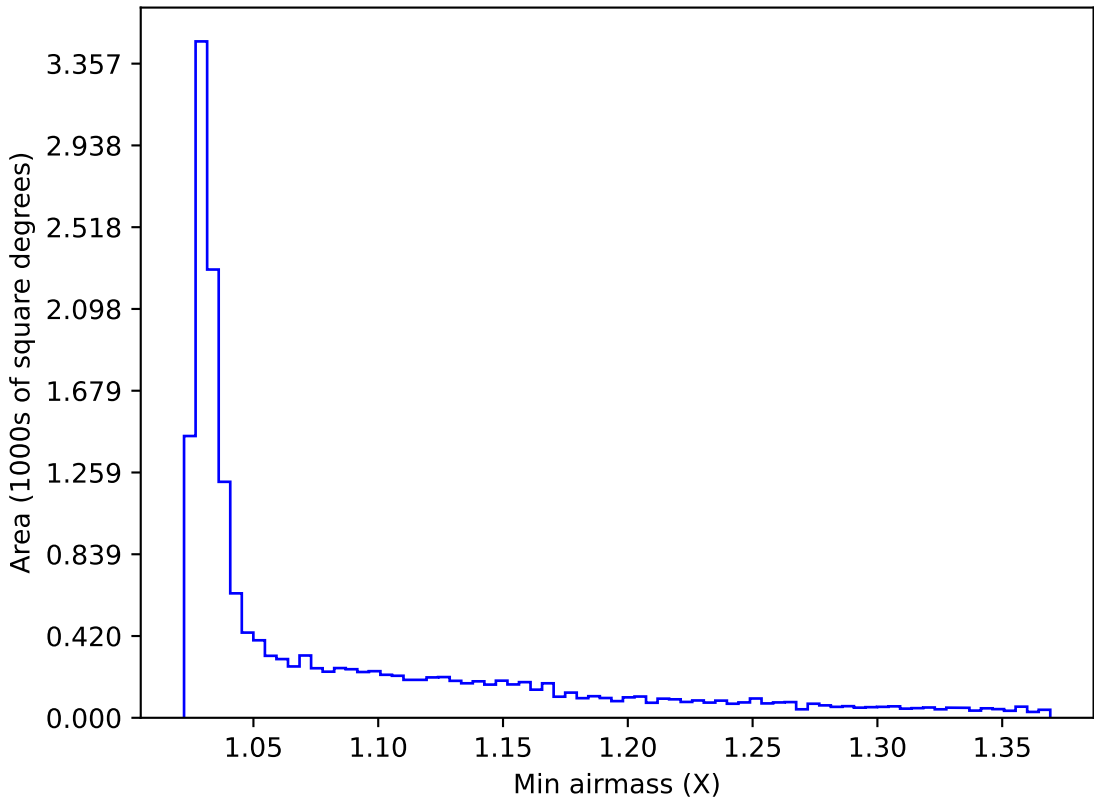
ddf_acor_sf30_lsf40_lsr20_v3.4_10yrs WFD y band: Min airmass
