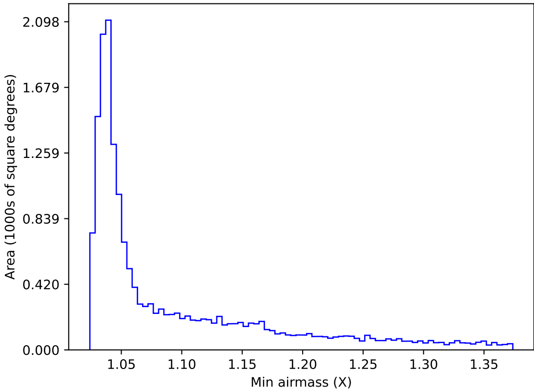
ddf_acor_sf30_lsf40_lsr20_v3.4_10yrs WFD u band: Min airmass
