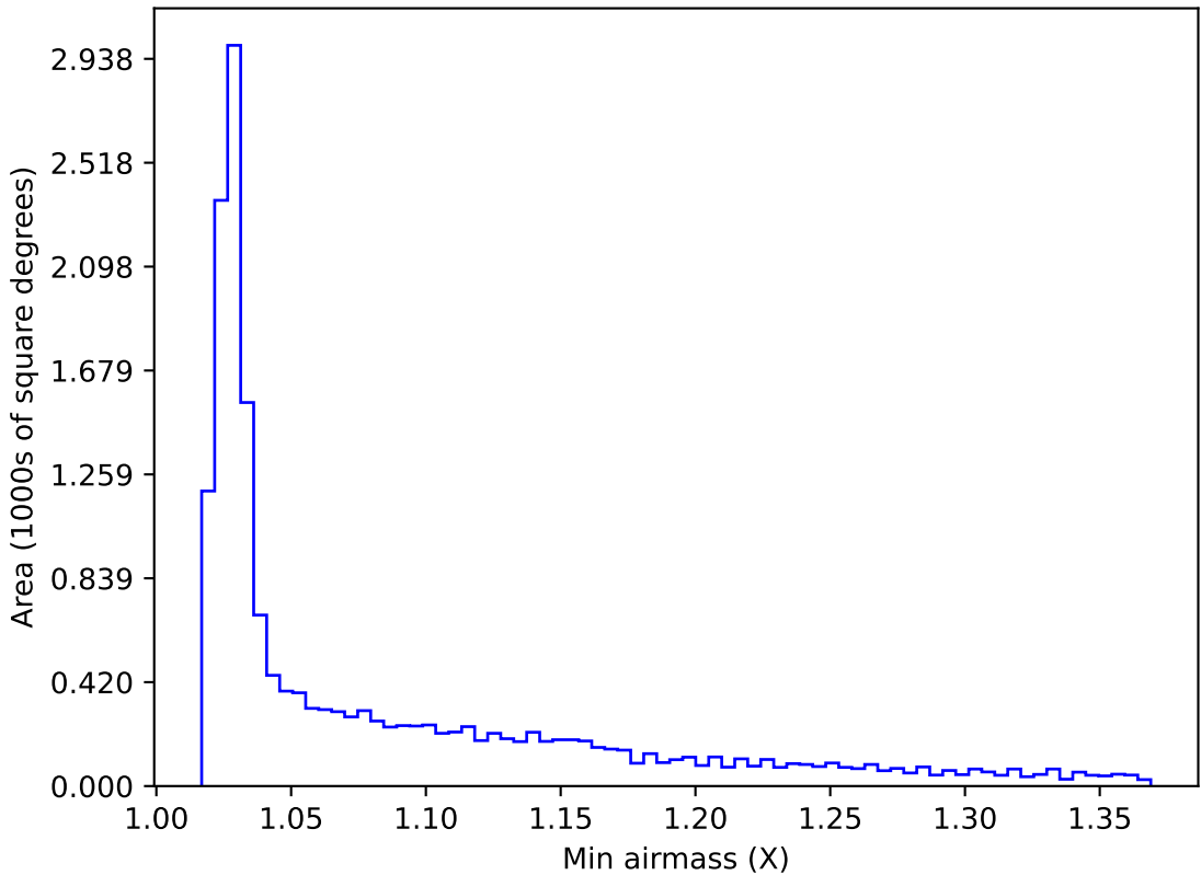
ddf_acor_sf30_lsf40_lsr20_v3.4_10yrs WFD r band: Min airmass
