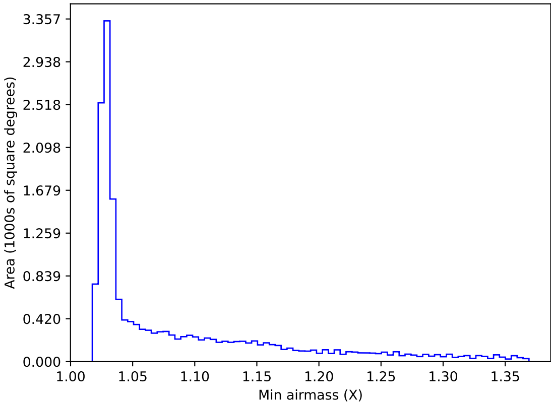
ddf_acor_sf30_lsf40_lsr20_v3.4_10yrs WFD i band: Min airmass
