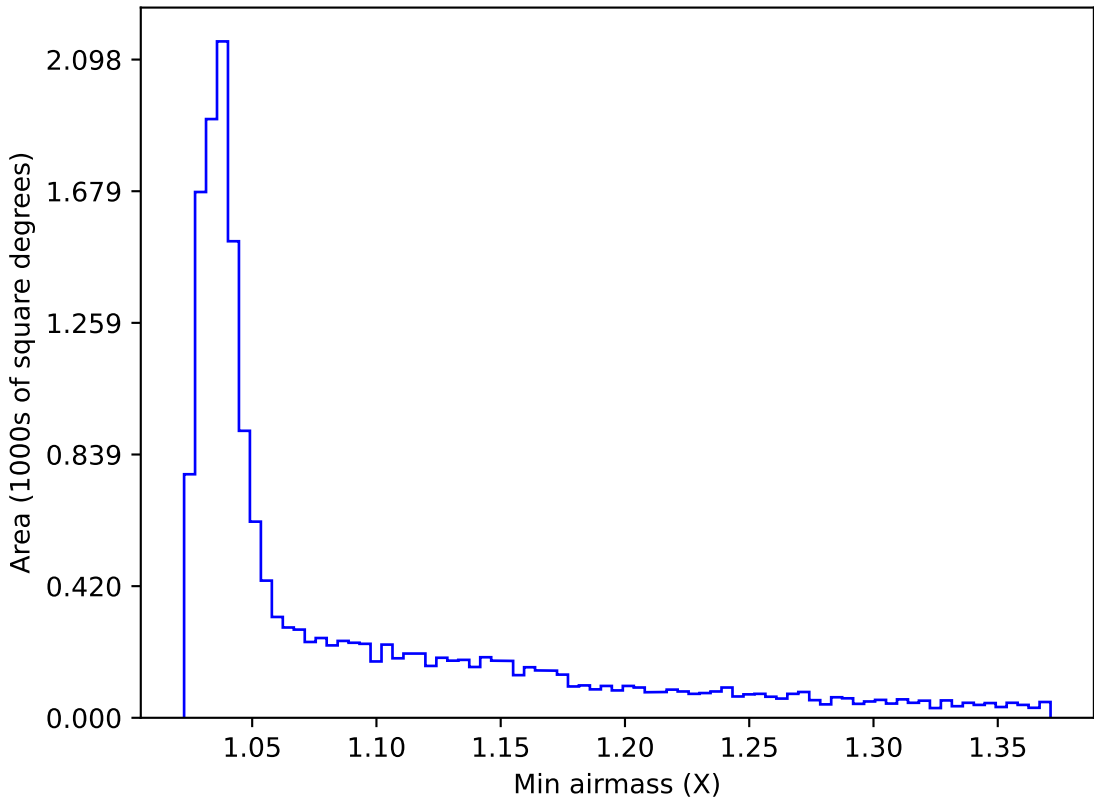
ddf_acor_sf30_lsf40_lsr20_v3.4_10yrs WFD g band: Min airmass
