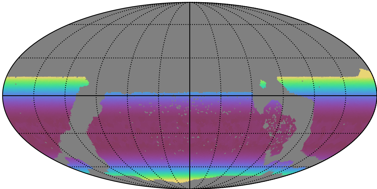
ddf_acor_sf30_lsf40_lsr20_v3.4_10yrs WFD all bands: Min airmass
