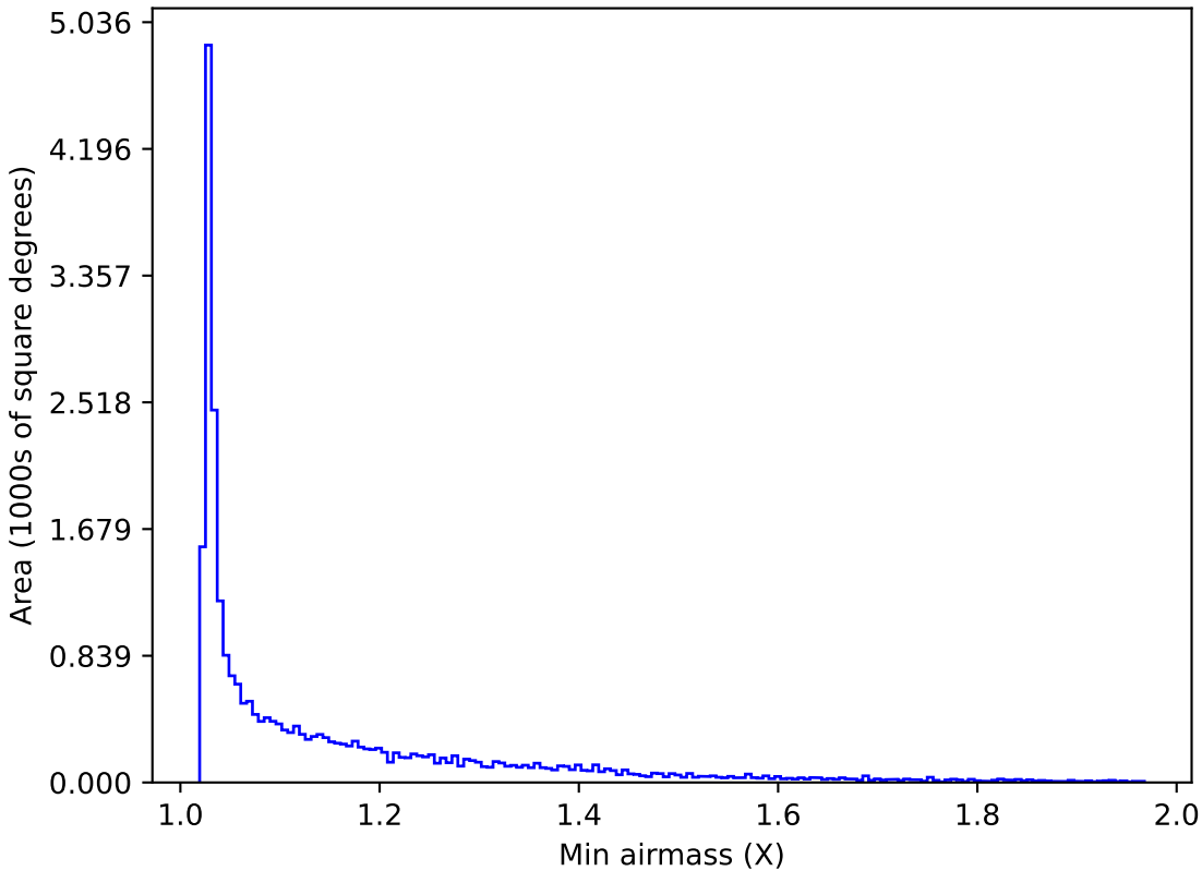
ddf_acor_sf30_lsf40_lsr20_v3.4_10yrs All sky z band: Min airmass
