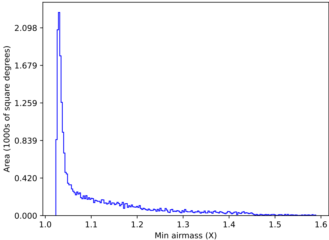
ddf_acor_sf30_lsf40_lsr20_v3.4_10yrs All sky y band: Min airmass
