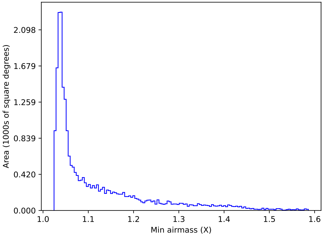
ddf_acor_sf30_lsf40_lsr20_v3.4_10yrs All sky u band: Min airmass
