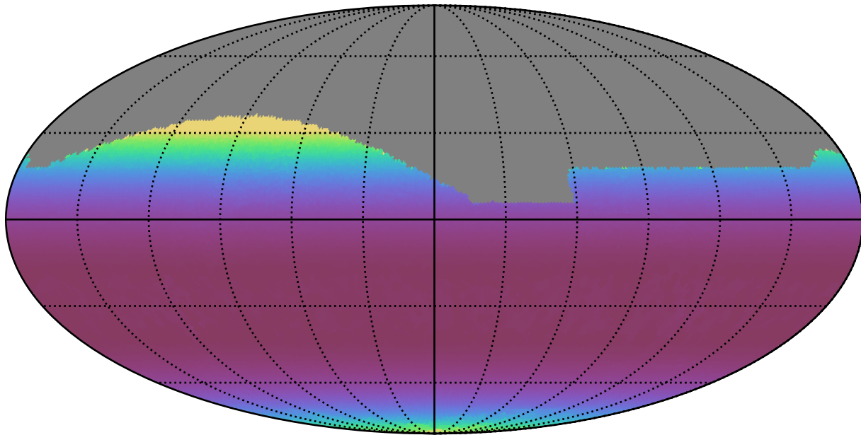
ddf_acor_sf30_lsf40_lsr20_v3.4_10yrs All sky r band: Min airmass
