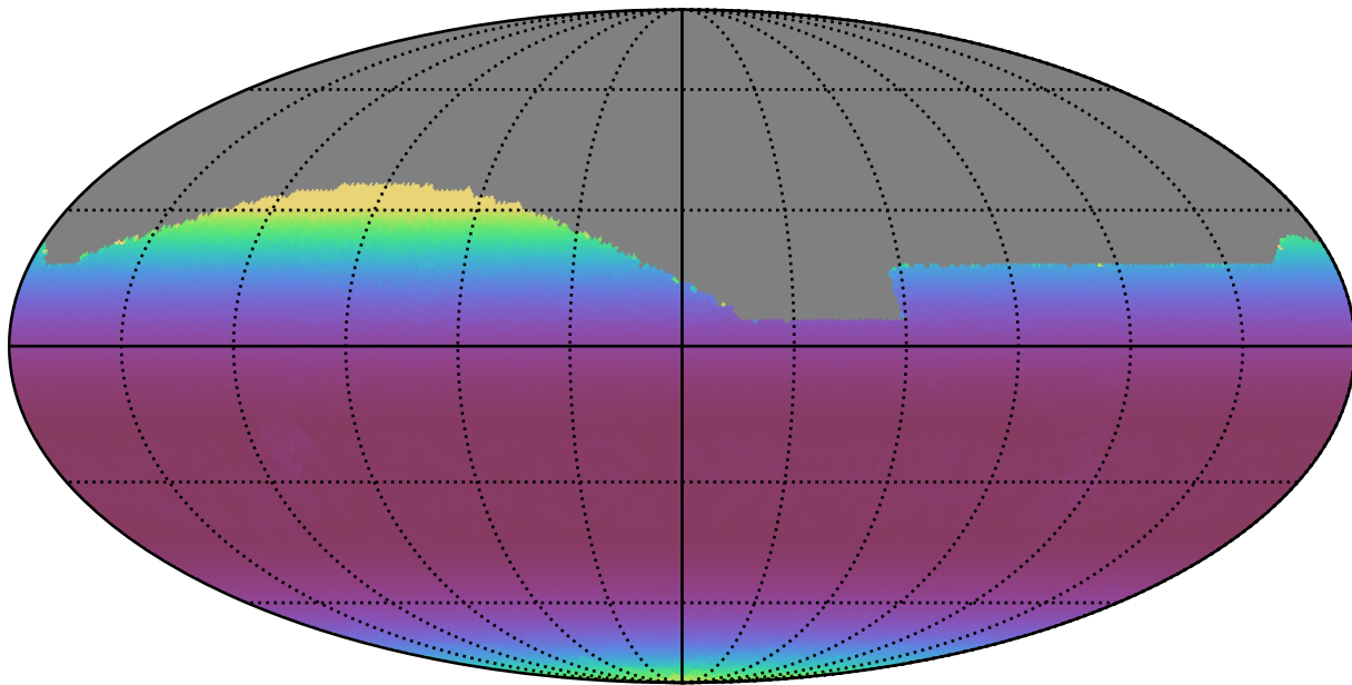
ddf_acor_sf30_lsf40_lsr20_v3.4_10yrs All sky i band: Min airmass
