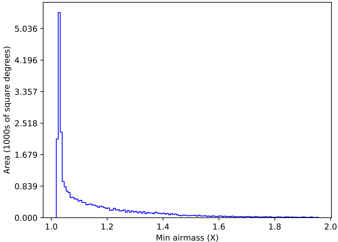
ddf_acor_sf30_lsf40_lsr20_v3.4_10yrs All sky i band: Min airmass
