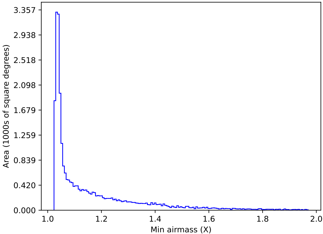
ddf_acor_sf30_lsf40_lsr20_v3.4_10yrs All sky g band: Min airmass
