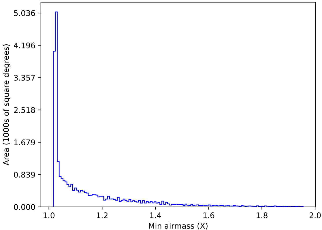
ddf_acor_sf30_lsf40_lsr20_v3.4_10yrs All sky all bands: Min airmass
