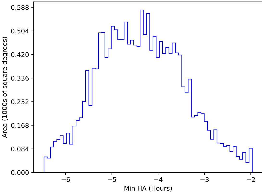
ddf_acor_sf30_lsf40_lsr20_v3.4_10yrs WFD z band: Min HA
