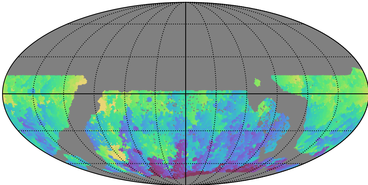
ddf_acor_sf30_lsf40_lsr20_v3.4_10yrs WFD u band: Min HA
