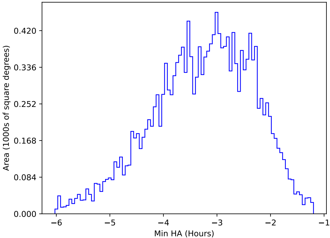
ddf_acor_sf30_lsf40_lsr20_v3.4_10yrs WFD u band: Min HA
