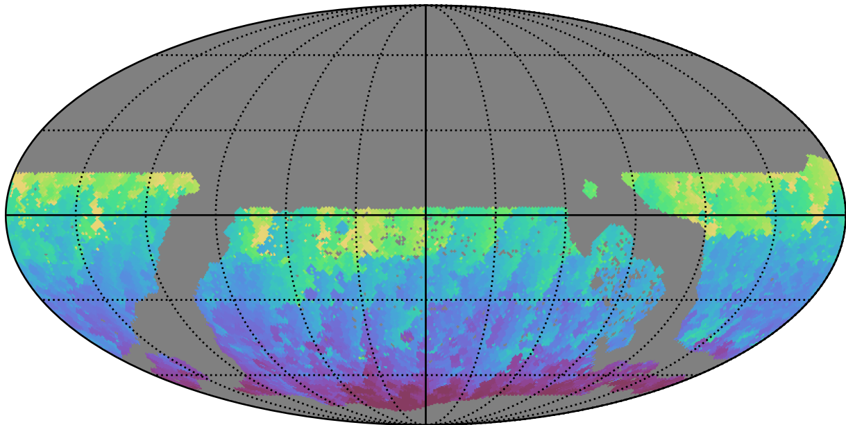
ddf_acor_sf30_lsf40_lsr20_v3.4_10yrs WFD g band: Min HA
