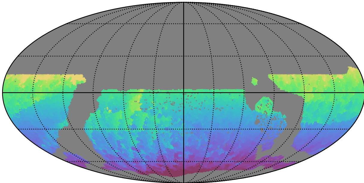
ddf_acor_sf30_lsf40_lsr20_v3.4_10yrs WFD all bands: Min HA
