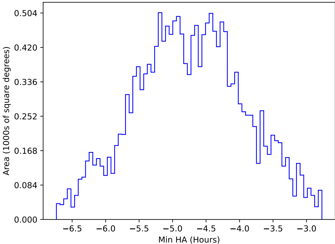
ddf_acor_sf30_lsf40_lsr20_v3.4_10yrs WFD all bands: Min HA
