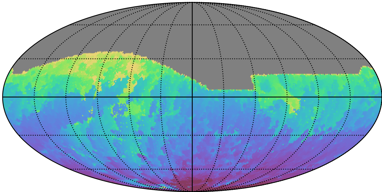
ddf_acor_sf30_lsf40_lsr20_v3.4_10yrs All sky z band: Min HA
