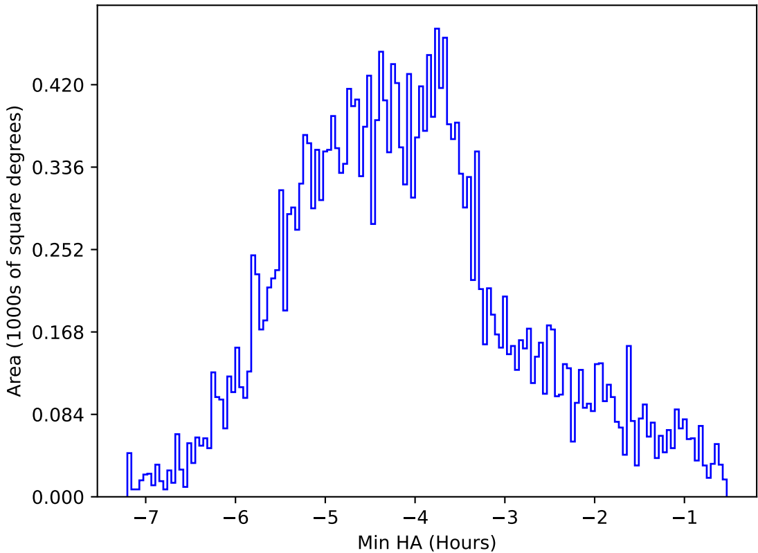
ddf_acor_sf30_lsf40_lsr20_v3.4_10yrs All sky z band: Min HA
