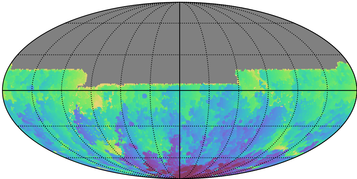
ddf_acor_sf30_lsf40_lsr20_v3.4_10yrs All sky u band: Min HA
