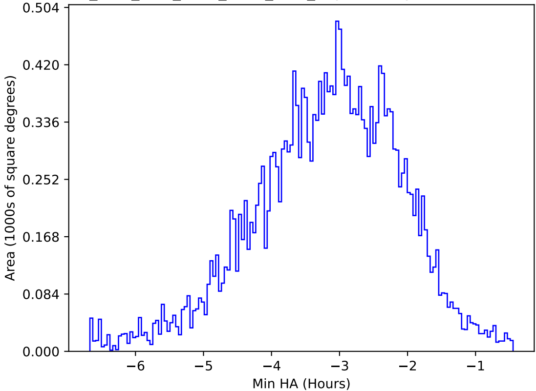
ddf_acor_sf30_ls40_lsr20_v3.4_10yrs All sky u band: Min HA
