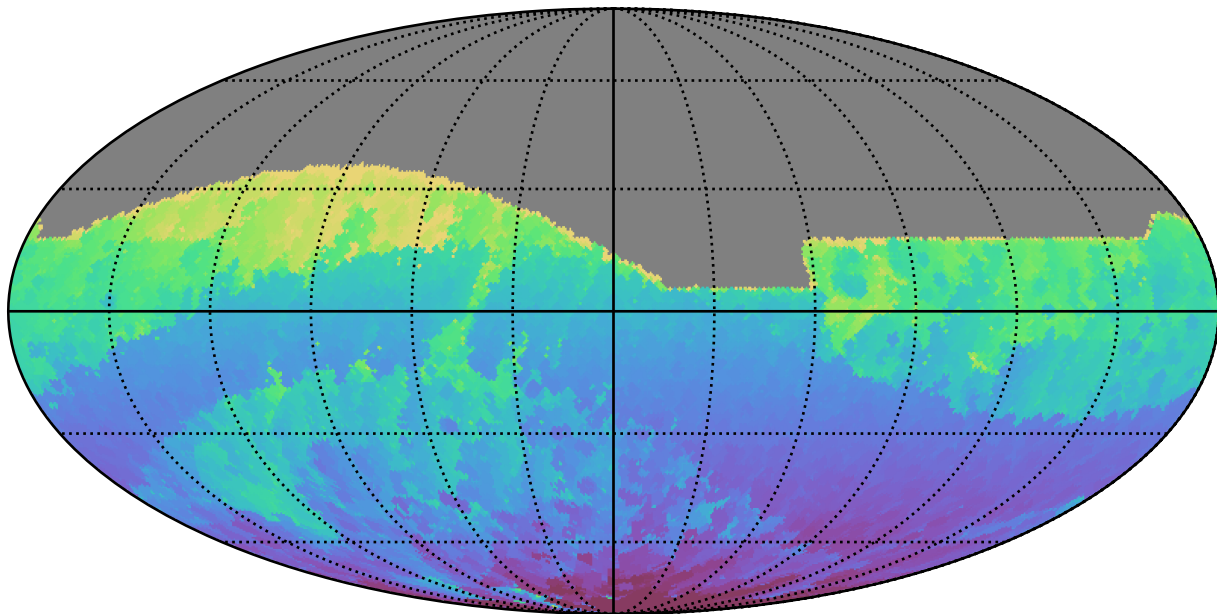
ddf_acor_sf30_lsf40_lsr20_v3.4_10yrs All sky r band: Min HA
