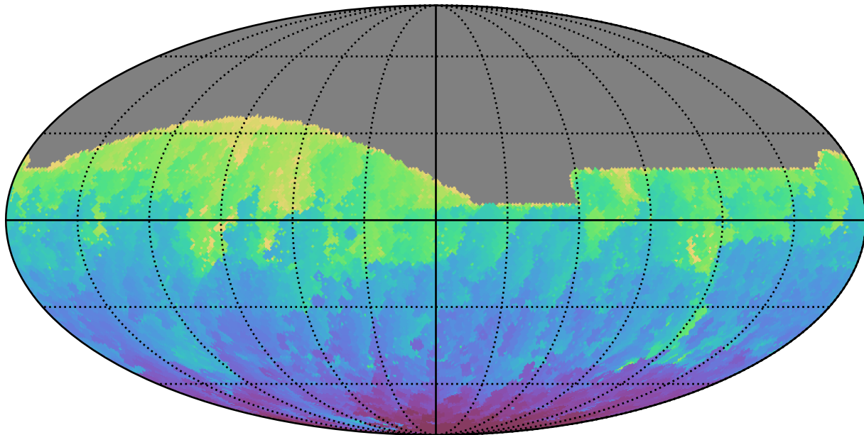
ddf_acor_sf30_lsf40_lsr20_v3.4_10yrs All sky g band: Min HA
