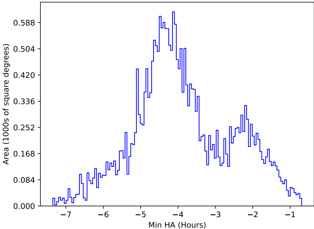
ddf_acor_sf30_ls40_lsr20_v3.4_10yrs All sky g band: Min HA
