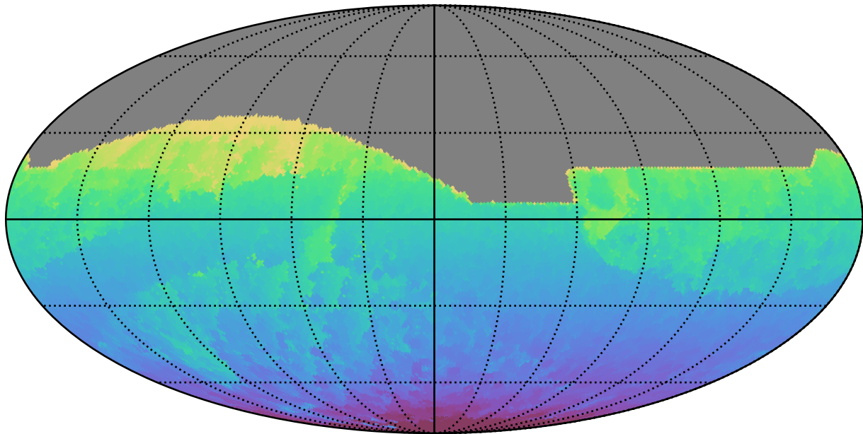
ddf_acor_sf30_lsf40_lsr20_v3.4_10yrs All sky all bands: Min HA
