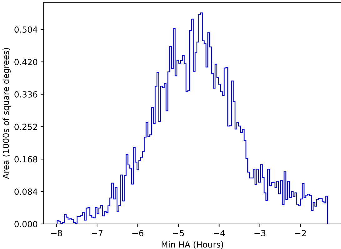
ddf_acor_sf30_lsf40_lsr20_v3.4_10yrs All sky all bands: Min HA
