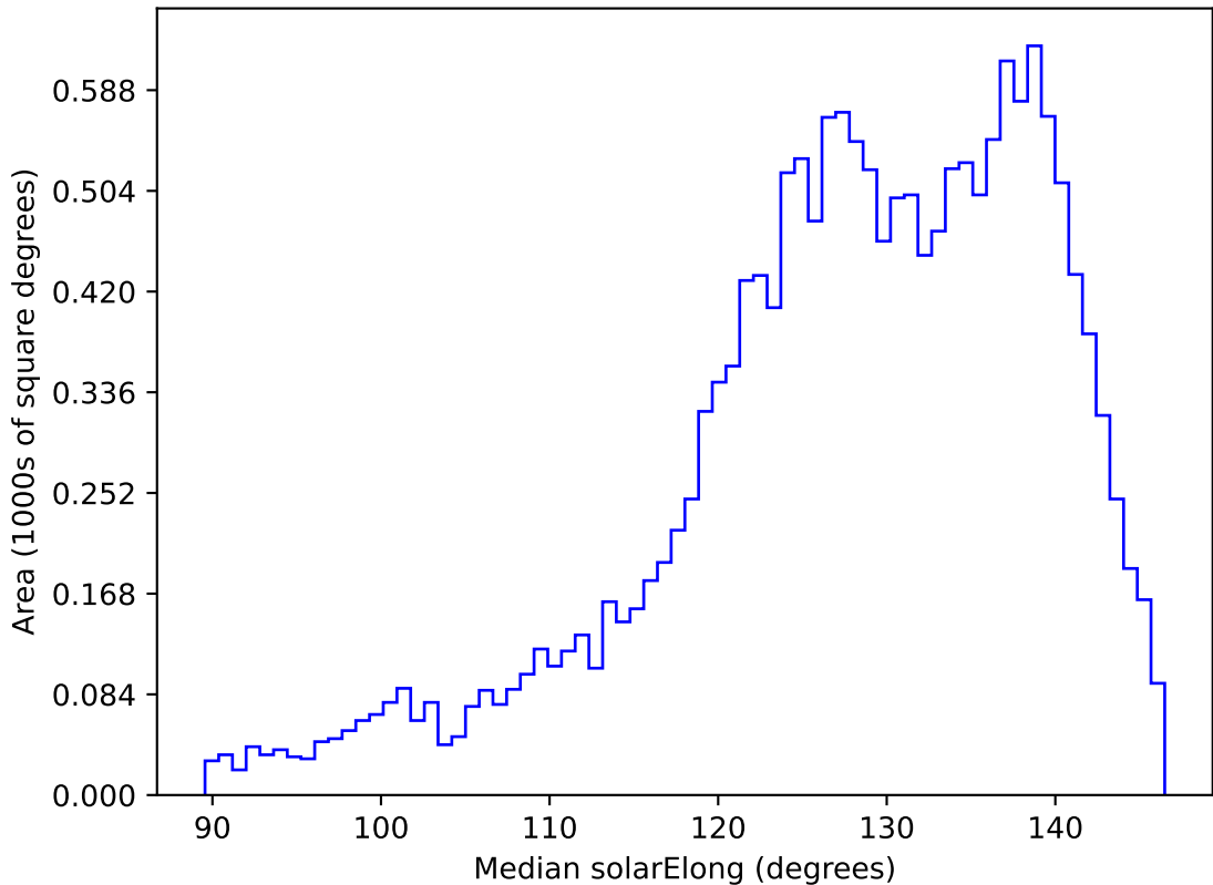
ddf_acor_sf30_lsf40_lsr20_v3.4_10yrs WFD z band: Median solarElong
