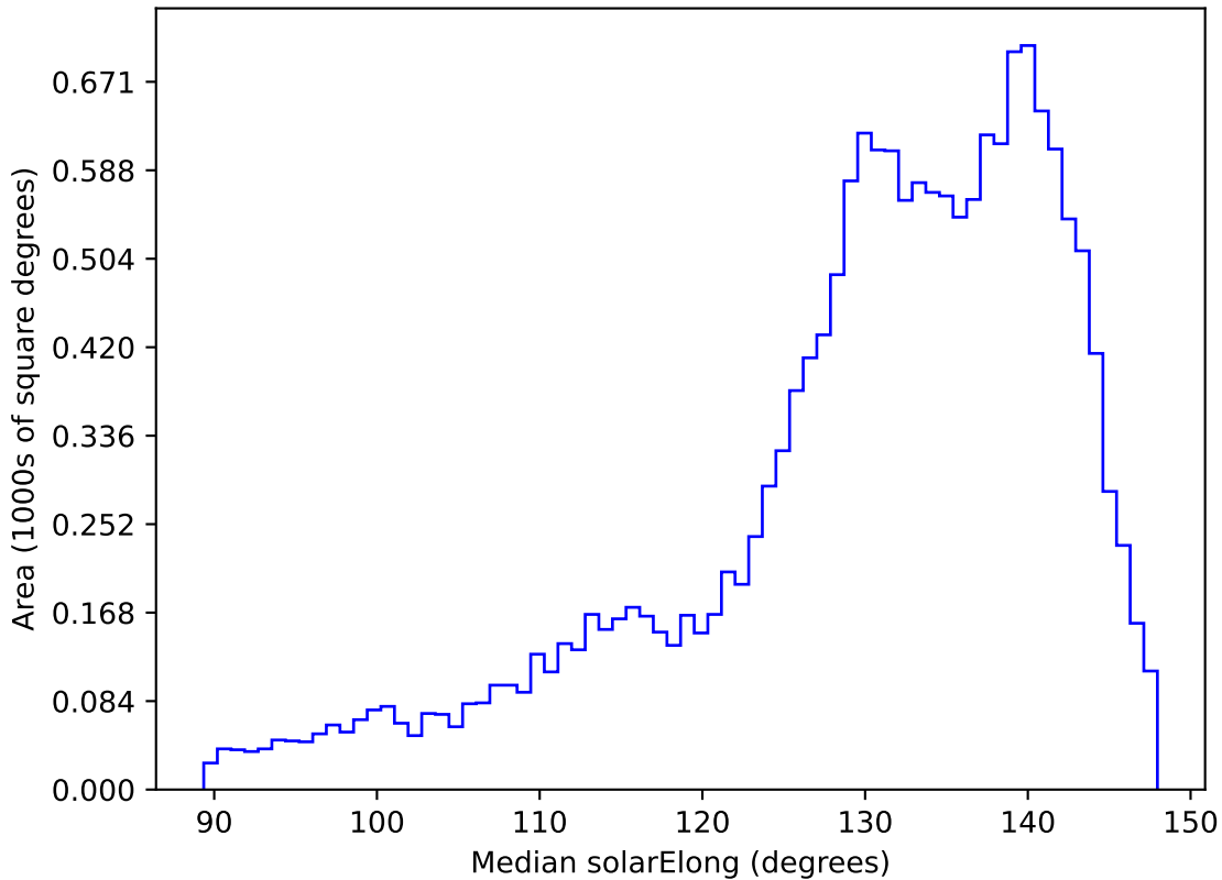
ddf_acor_sf30_lsf40_lsr20_v3.4_10yrs WFD y band: Median solarElong
