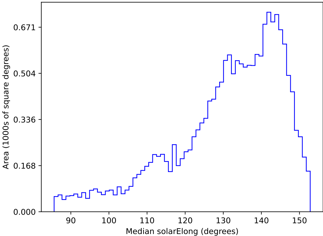
ddf_acor_sf30_lsf40_lsr20_v3.4_10yrs WFD u band: Median solarElong
